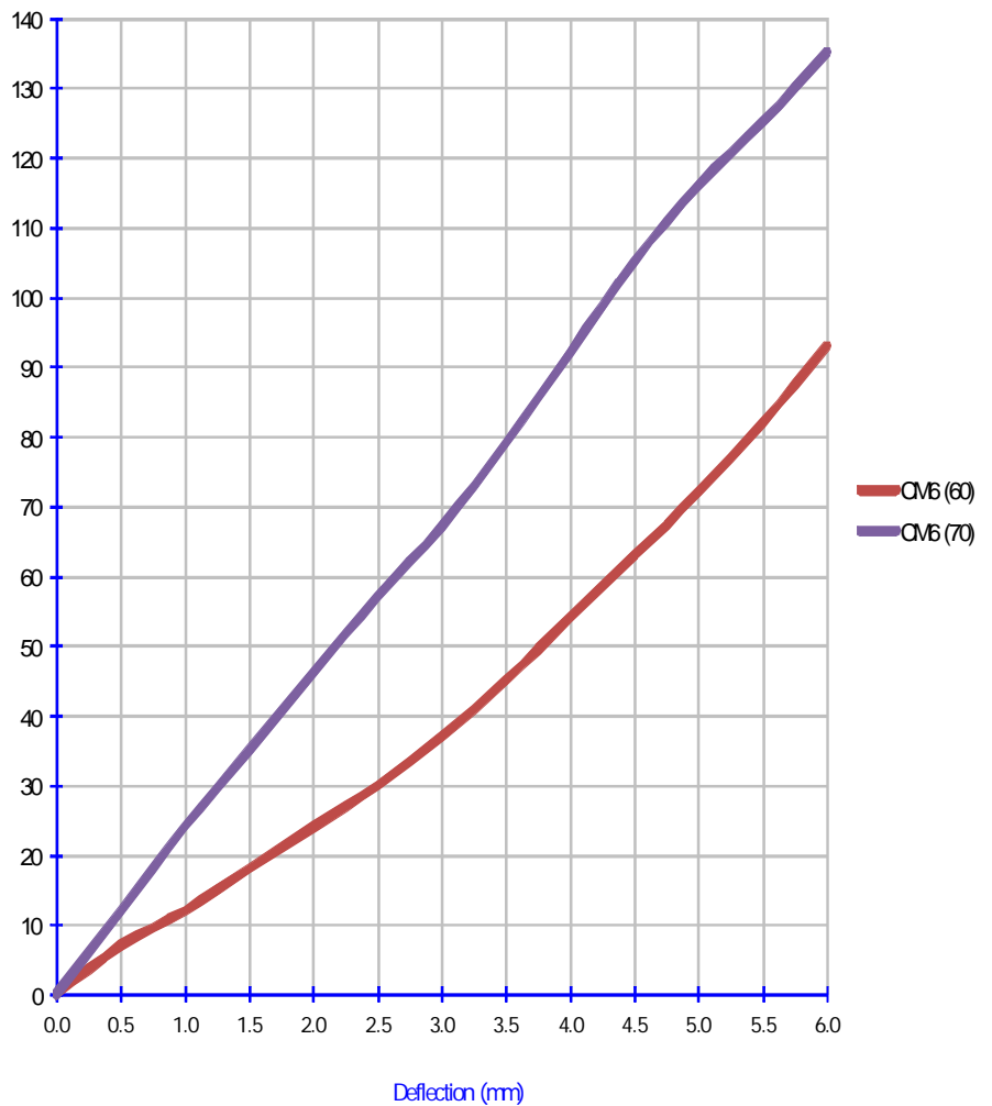
Graph: 1. Static Axial Vertical Load[kg] (A-direction) versus Deflection[mm]
