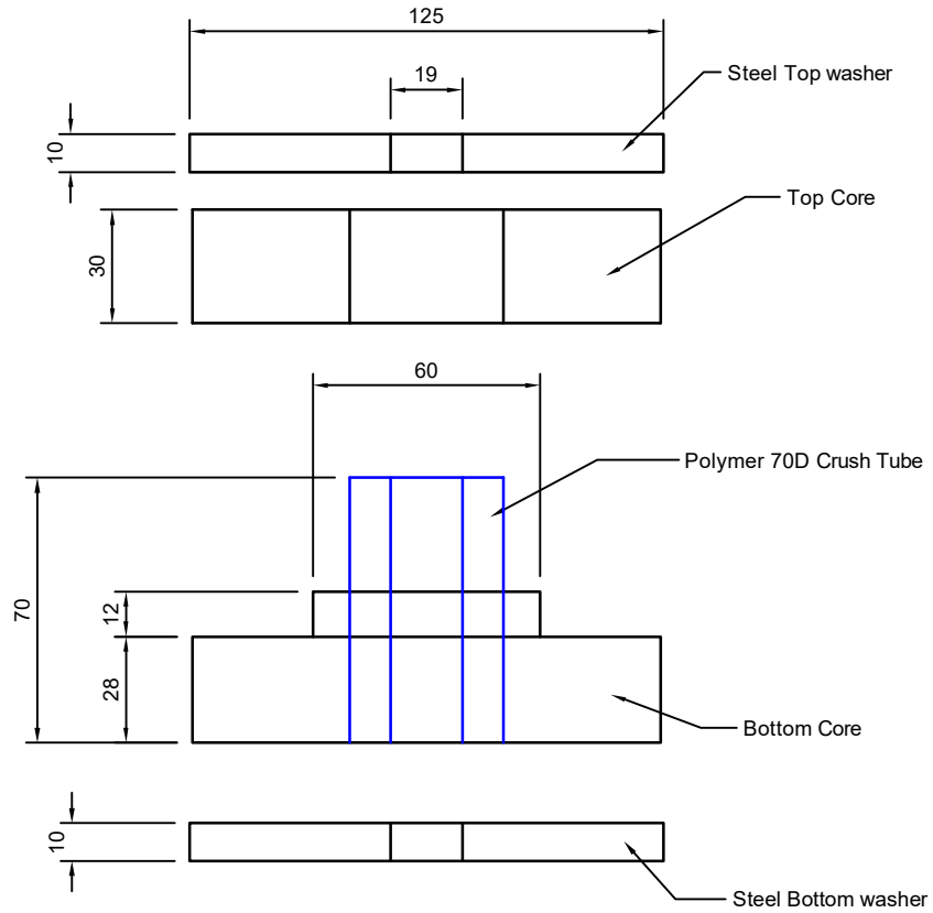
MT125601234 Components
