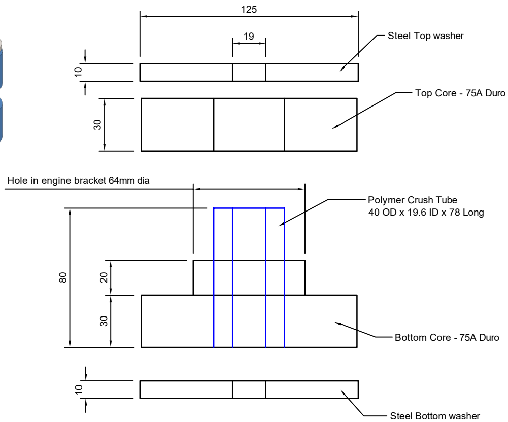
MT1255919 - Mount Components
