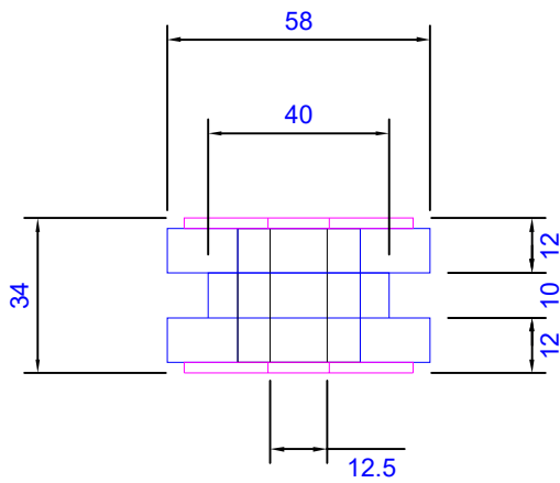
MT58401012 Mount Assy (Old Part No.: MT405822)
