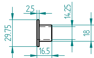
Item 4: 14mm to 18mm steel bush kit supplied
