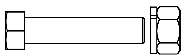
Item 2: \frac{7}{16} " UNF x 2" Hex Bolt, Nut and Spring Washer
