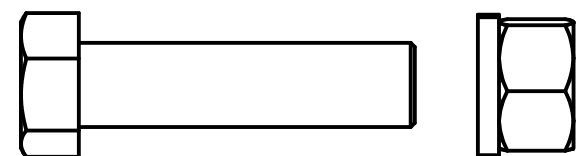
Item 2: 7/8" UNC x 3 1/2" Hex Head Bolt, Nut and Spring Washer
