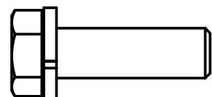
Item 3: 3/8" UNF x 1 1/4" Hex Bolt and Spring Washer
