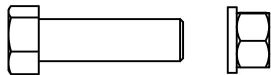
Item 2: 3/8" UNF x 1 1/2" Hex Bolt, Nut and Spring Washer
